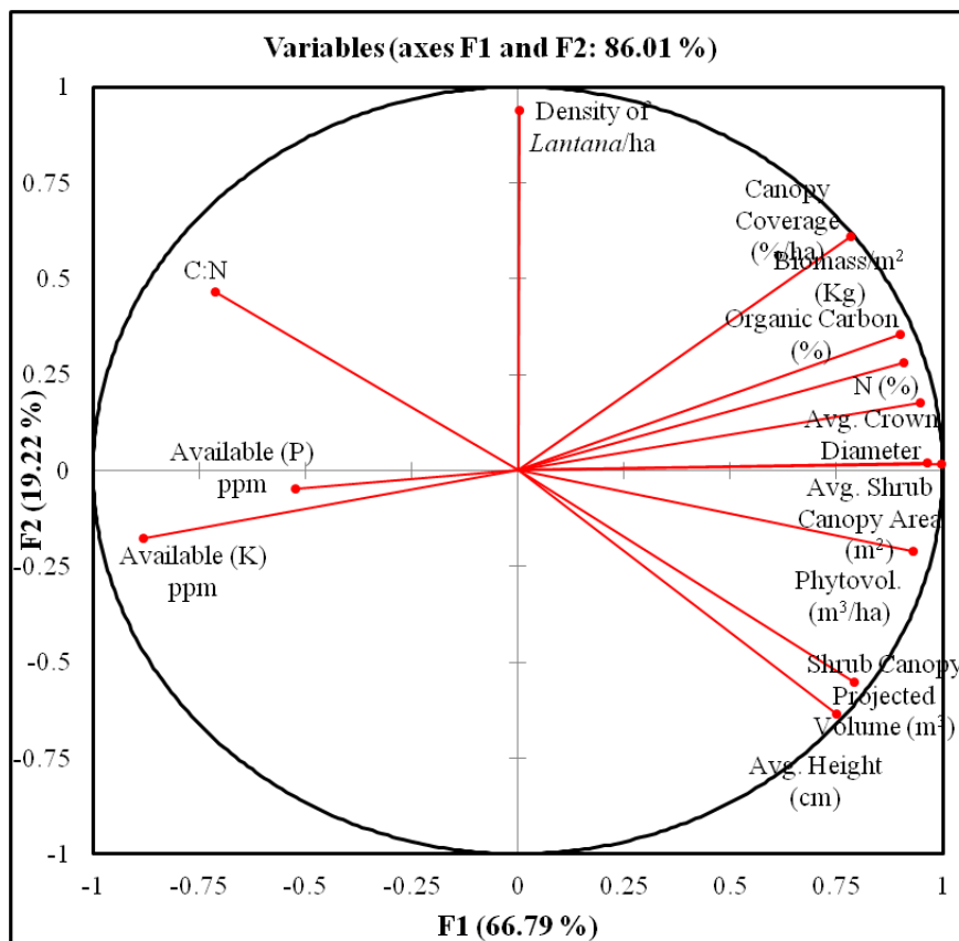
Figure 3. Principal component analysis (PCA) representation of soil attributes and calculated and measured attributes of Lantana from different sites (n = 20) of Doon Valley
