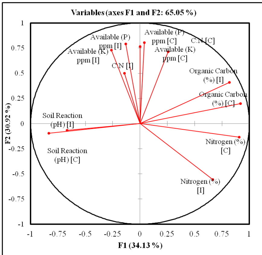
Figure 2. Principal component analysis (PCA) representation of soil attributes from both control and invaded sites of Lantana (n = 20) from Doon Valley.
